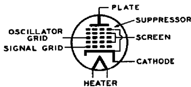
PENTAGRID MIXER
