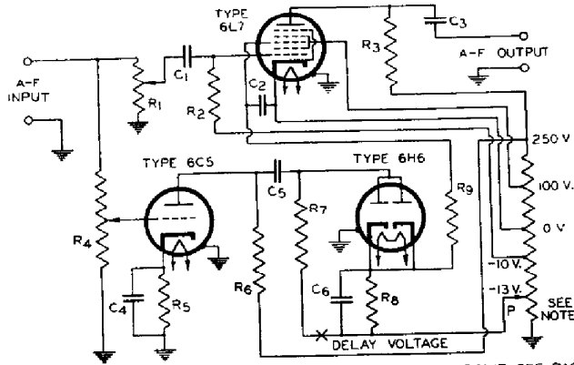
VOLUME EXPANDER USING TYPE 6L7 FOR USE IN A PHONOGRAPH AMPLIFIER
