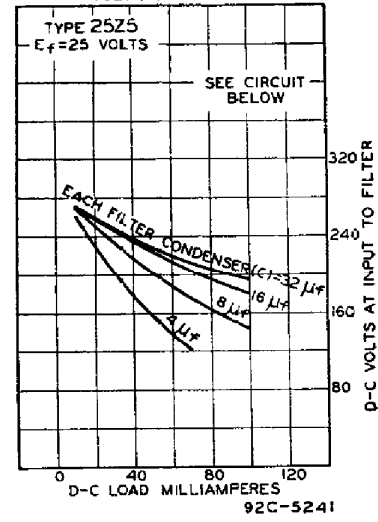
OPERATION CHARACTERISTICS VOLTAGE DOUBLER
