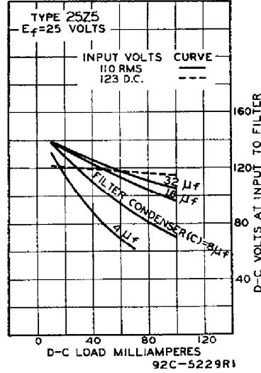
OPERATION CHARACTERISTICS HALF-WAVE RECTIFIER
