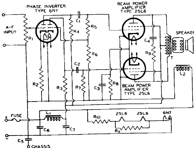
AUDIO AMPLIFIER FOR USE ON 115-VOLT D-C LINE CLASS A 1 - POWER OUTPUT, 4 WATTS*
