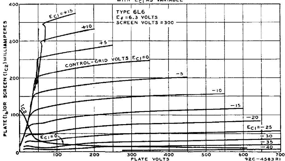
AVERAGE PLATE CHARACTERISTICS WITH E_{C1} AS VARIABLE
