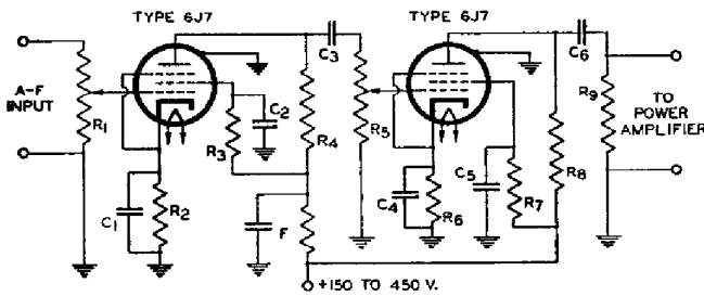
NON-MOTORBOATING RESISTANCE-COUPLED AMPLIFIER VOLTAGE GAIN = 9000
