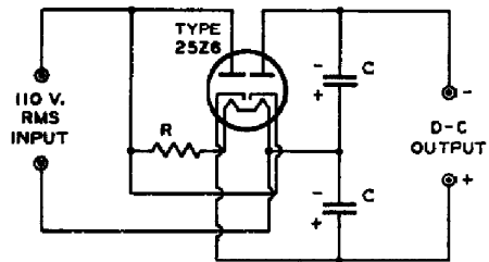
VOLTAGE-DOUBLER CIRCUIT
