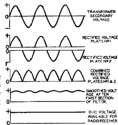
FULL-WAVE RECTIFICATION
