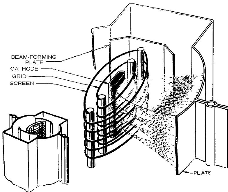
INTERNAL STRUCTURE OF BEAM POWER TUBE
