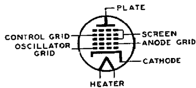
PENTAGRID CONVERTER
