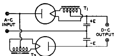
T 1 , T 2 = SEPARATE FILAMENT TRANSFORMER WINDINGS.
