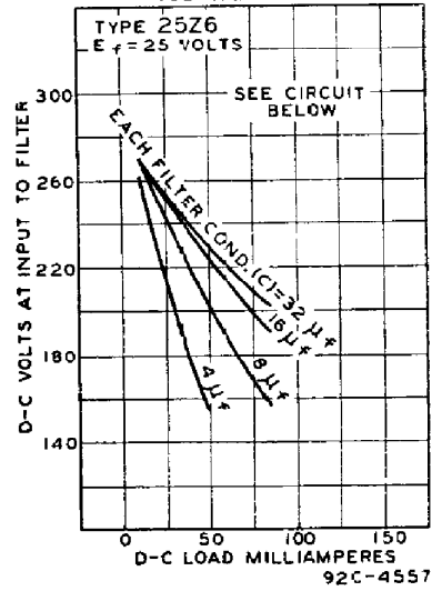
OPERATION CHARACTERISTICS VOLTAGE DOUBLER
