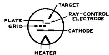
ELECTRON-RAY TUBE
