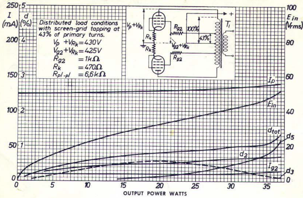
FIG. 1 PERFORMANCE OF TWO 6CA7 IN PUSH-PULL WITH DISTRIBUTED LOAD CONDITIONS. SCREEN-GRID TAPPING AT 43% OF PRIMARY TURNS
