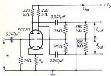
Circuit A
