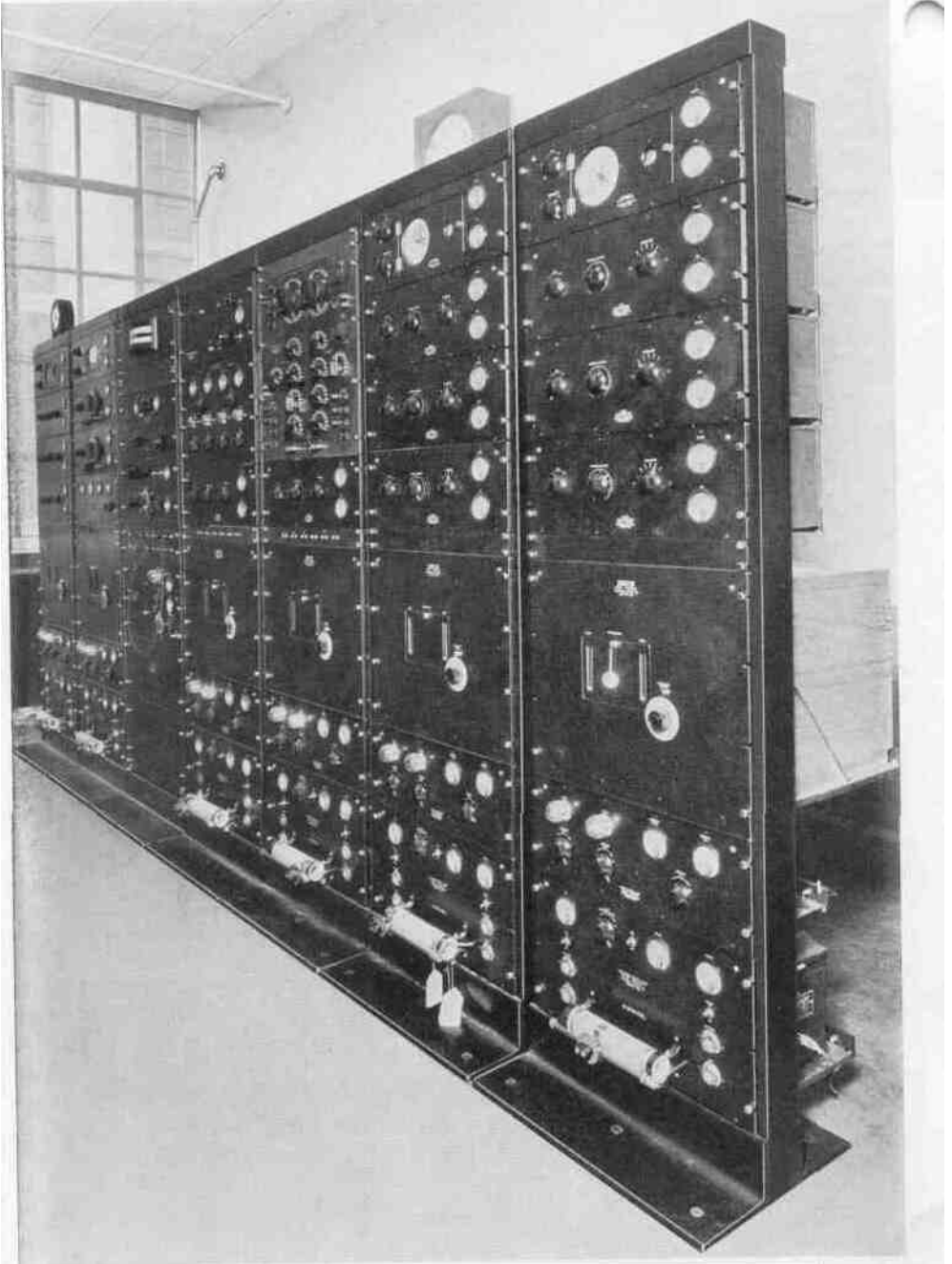
The General Radio Company's frequency-standards room. At the extreme left is a relay rack carrying the standard-frequency assembly we use for our own frequency measurements, and at the extreme right are two assemblies being tested before shipment to purchasers. The remainder is experimental equipment
