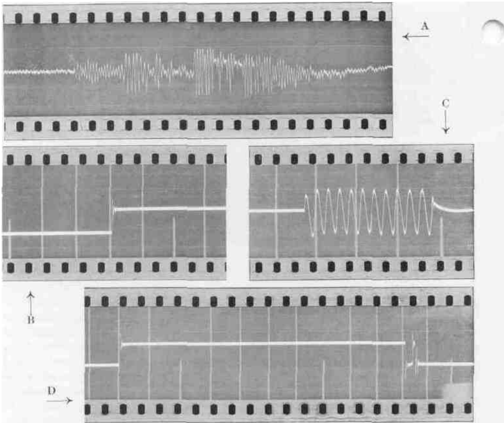
FIGURE 3. Typical records taken with the string oscillograph and camera. The vertical timing lines and the white spot (lower right corner of D ) were marked at 1/50th-second and 1-second intervals by a synchronous shutter. A is the record of a watch tick; B and D show the operation of a relay; C shows the starting and stopping of a vacuum-tube oscillator. Time increases from left to right
