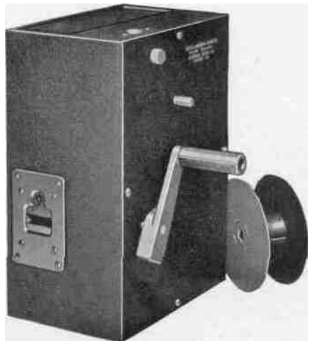
FIGURE 4. The Type 408 Oscillograph Camera
