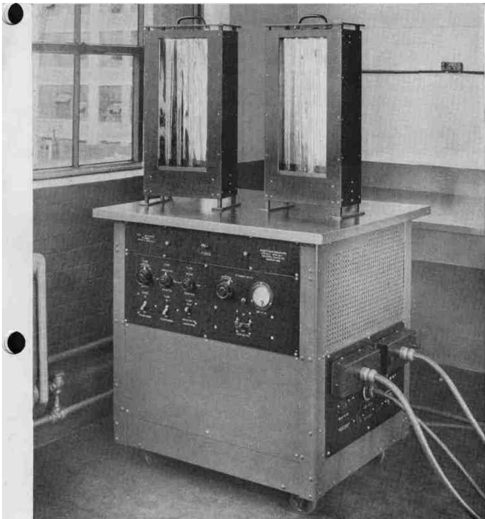
The power supply and the control equipment for the TYPE 521-A Edgerton Stroboscope are contained inside the truck. The two lamp banks on the table top can be moved anywhere within range of the cables at the right
