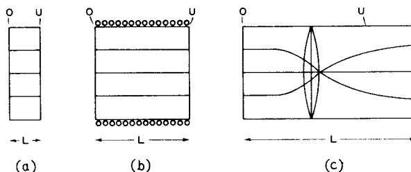
(a) SIMPLE ACCELERATING FIELD (b) UNIFORM ELECTRIC AND MAGNETIC FIELD (c) IMAGE TUBE
