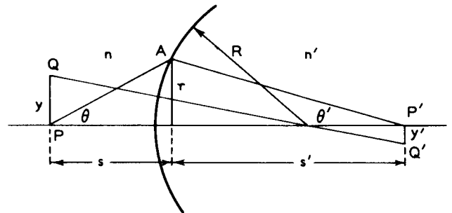
Fig. 3 - Refraction at a curved surface.
