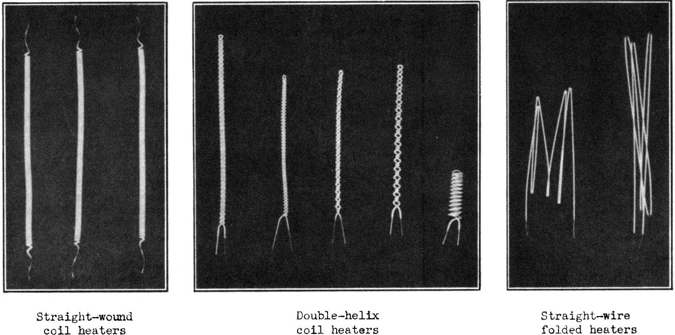
Fig. 4 - Types of heaters.
