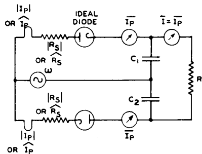
VOLTAGE-DOUBLING CIRCUIT
