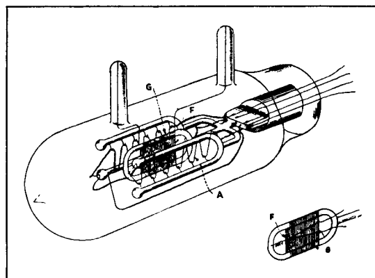
Fig. 4 - Tube constructed with filamentary electrodes.
