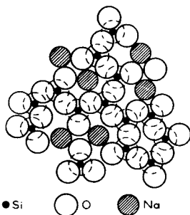
Fig. 1 - Schematic arrangement of atoms in a soda silica glass. (Courtesy of American Ceramic Society)
