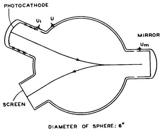
Fig. 14 - Image tube with mirror.
