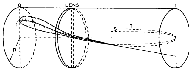
Fig. 5 - The image formation in a flat-cathode image tube.
