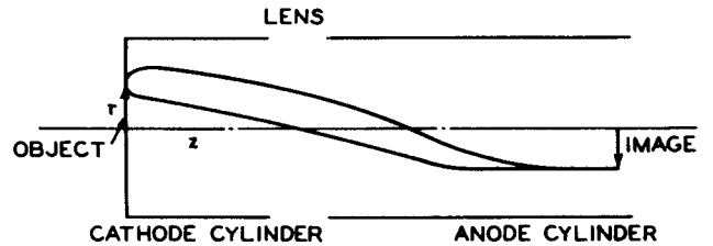
Fig. 17 - Cathode lens.
