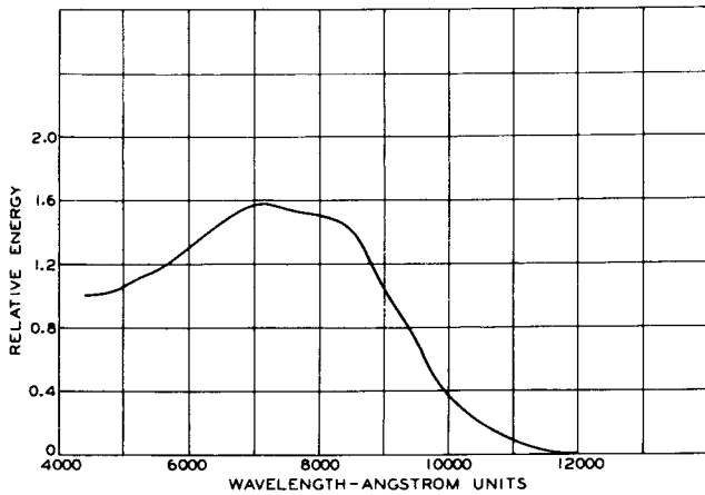
Fig. 21 - Spectral distribution curve for semitransparent photosurface having white-light sensitivity of 16-17 \mu /lumen.
