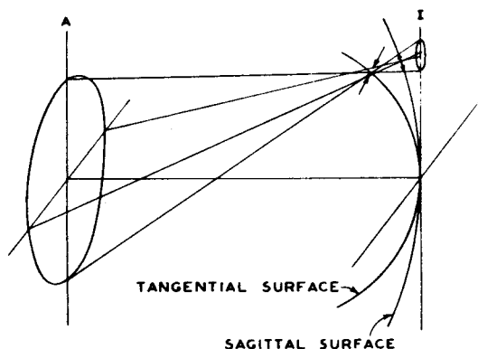
Fig. 4 - Curvature of field and astigmatism.
