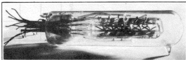
Fig. 9 - An experimental electrostatic secondary-emission multiplier.
